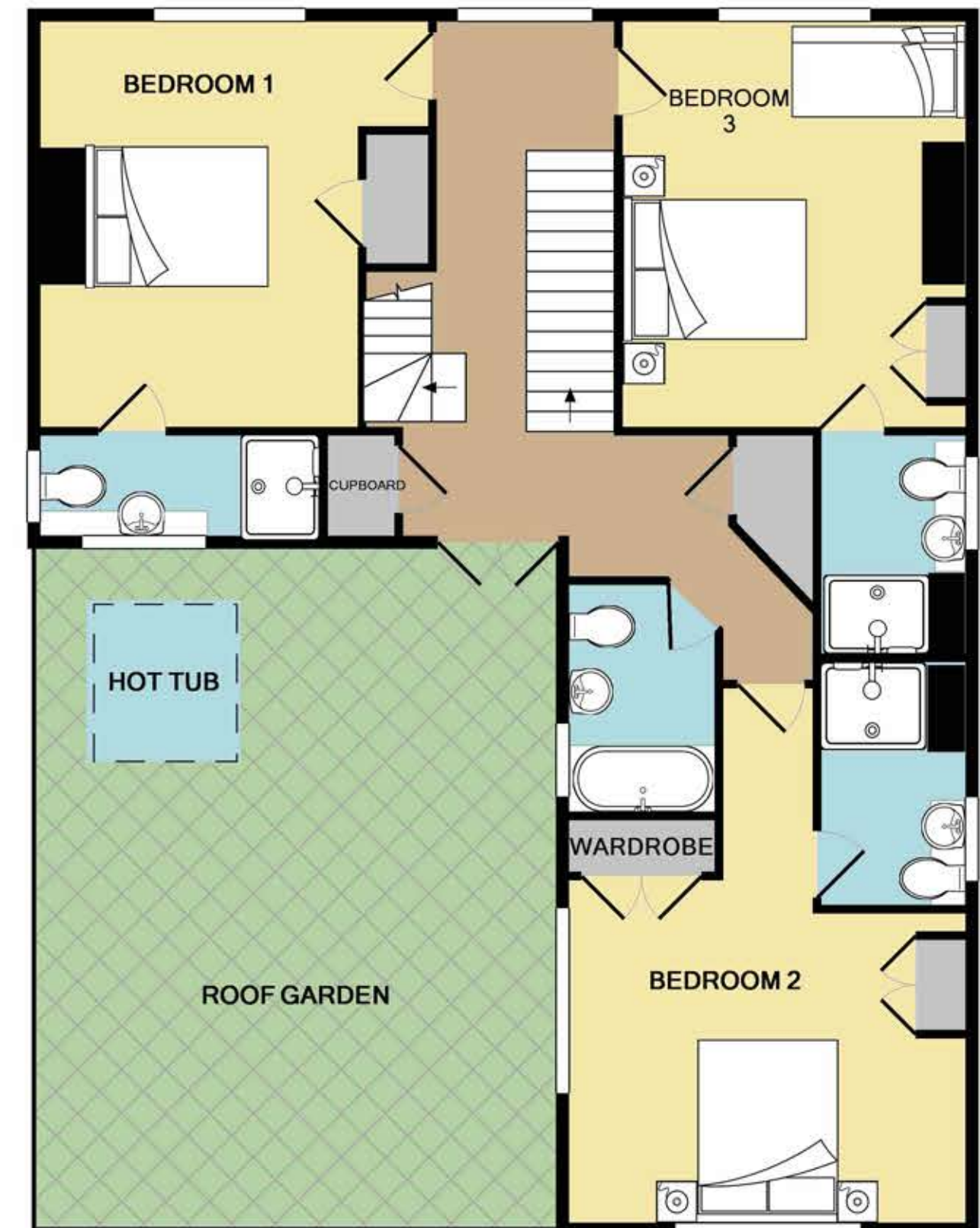
1ST FLOOR APPROX. FLOOR AREA 1087 SQ.FT. (101.0 SQ.M.)
